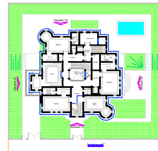
Second Floor Plan A = 366.18 m 2
